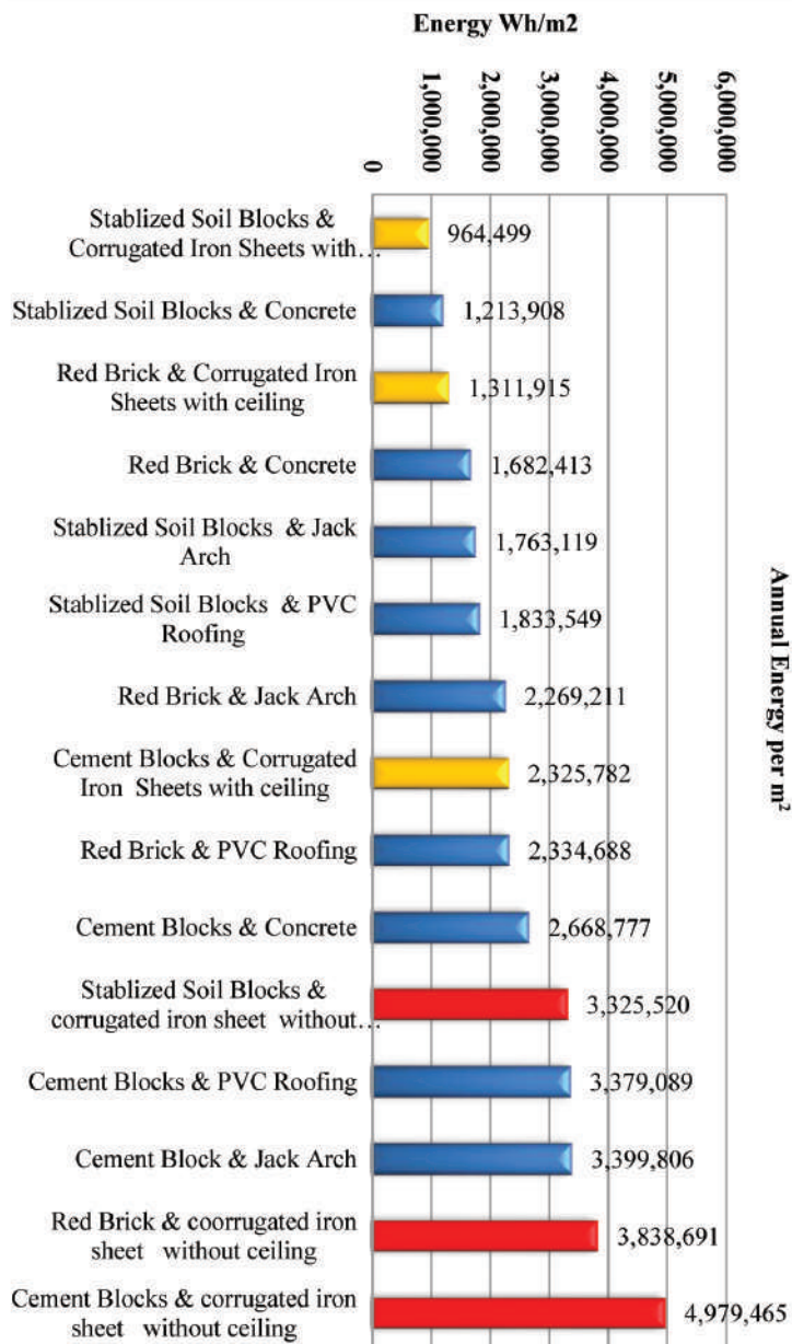
Fig. (2): Annual Energy that is needed to cool the house
