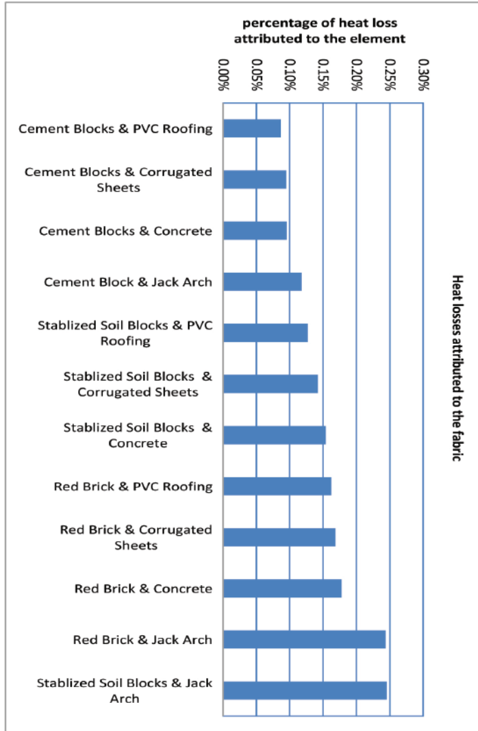
Fig. (6): Heat losses by the fabric for different alternatives
