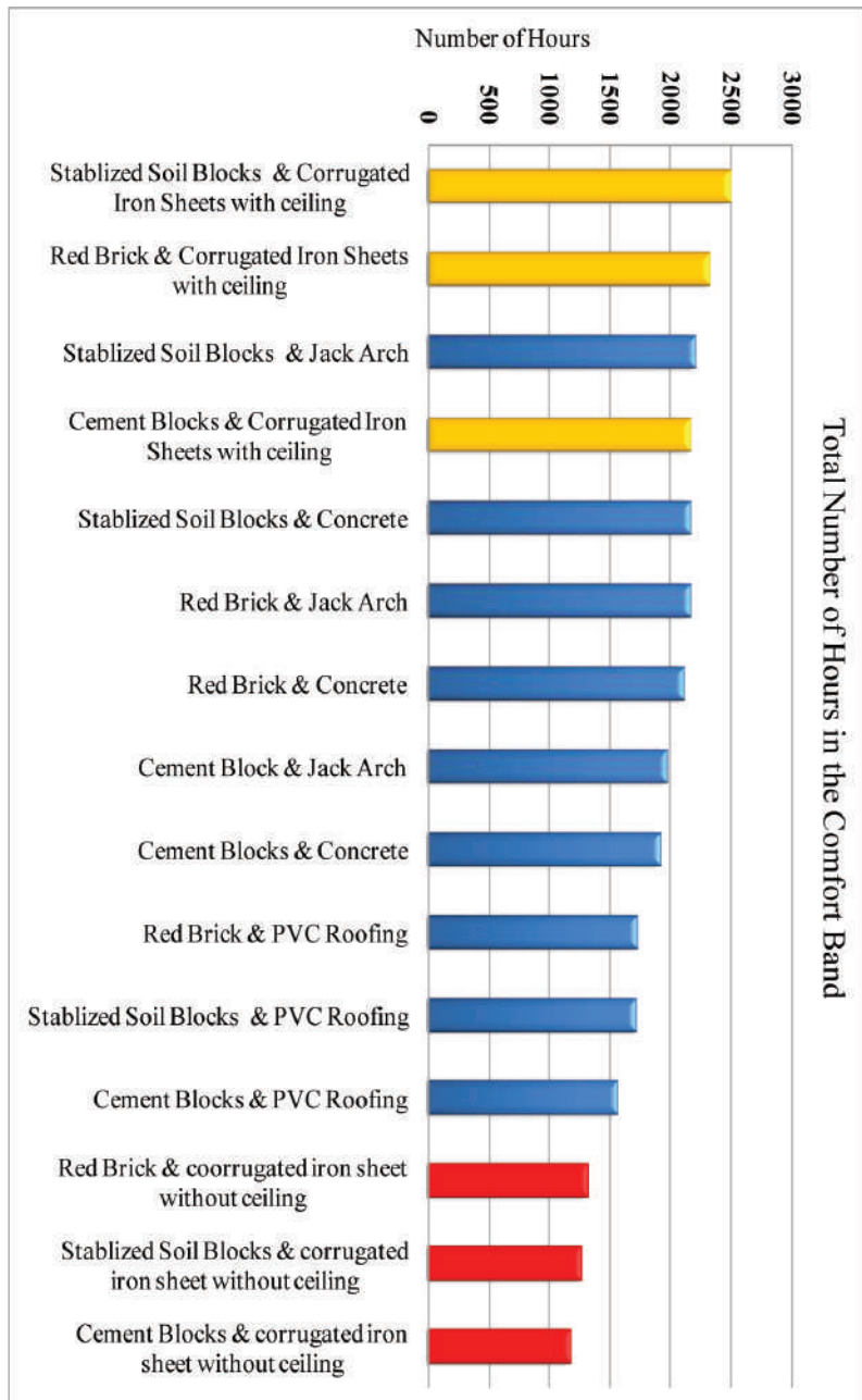
Fig. (3): Total number of hours inside the comfort band from the total hours of the year for each alternative
