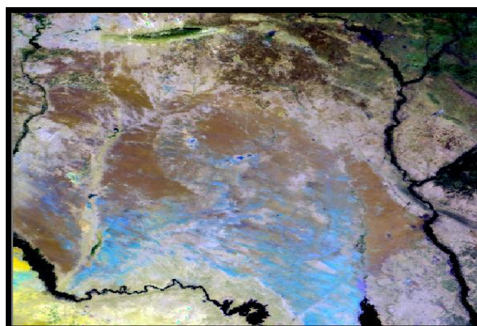
(B) MODIS comosite image in false color (R(7), G(6),B(3)) illustrate gypsiferous soil in turquoise blue color
