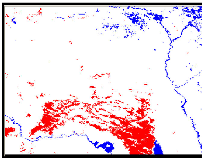
(D) MODIS unsupervised classification image at (2011-8-26) drought day, gypsiferous soil about 7.4%
