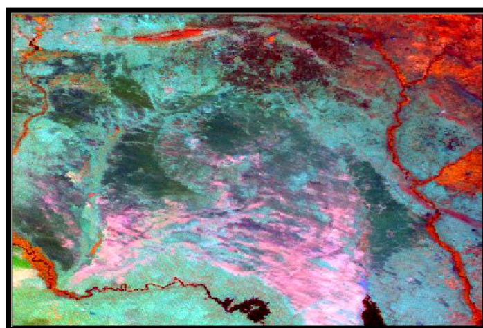
(C) MODIS composite in false color (R(band6-band7), G(2), B(3)) illustrate gypsiferous soil in magneta color.
