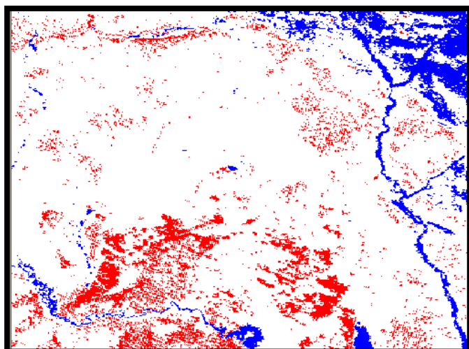
(B) MODIS unsupervised classification image at (2011-01-21) after rainfall in 17 days, gypsiferous soil about 8.9%
