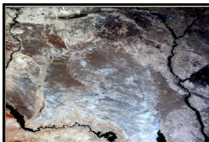
(A) MODIS composite image in true color (R(1), G(4),B(3)) illustrate gypsiferous soil in white color.
