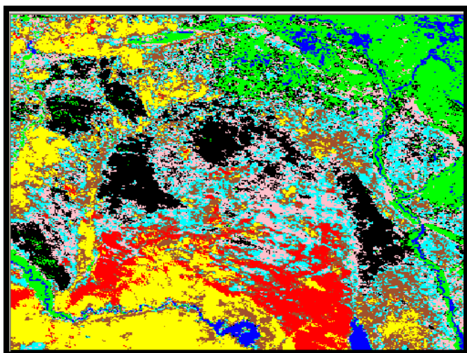
MODIS unsupervised classification image illustrating 8 classes in north-west Iraq.
