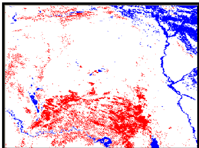
(A) MODIS Unsupervised classification image at (2011-01-07) after rainfall in 7 days, gypsiferous soil about 10.7%
