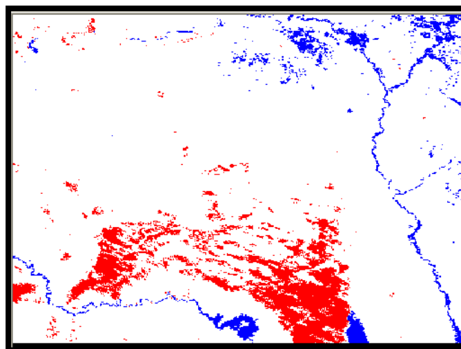
MODIS unsupervised classification image illustrating gypsiferous soil class in north-west Iraq that appear in red color.
