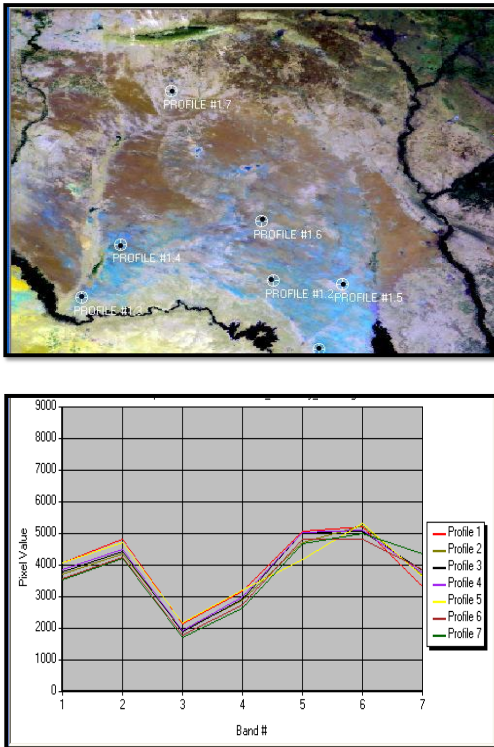
Fig. 3. MODIS spectral band profiles of seven locations dominated by gypsiferous soil (A) –note the peak in SWIR band 6 (1628-1652) nm, and the bsorption in Vis band 3(459-479) nm and SWIR band 7 (2105-2155) nm, (B)
