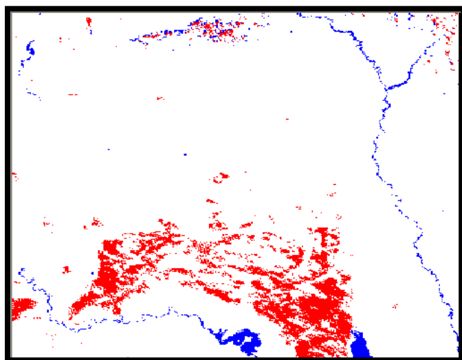
(C) MODIS unsupervised classification image at (2011-04-13) after dust storm in one day, gypsiferous soil about 6.38%
