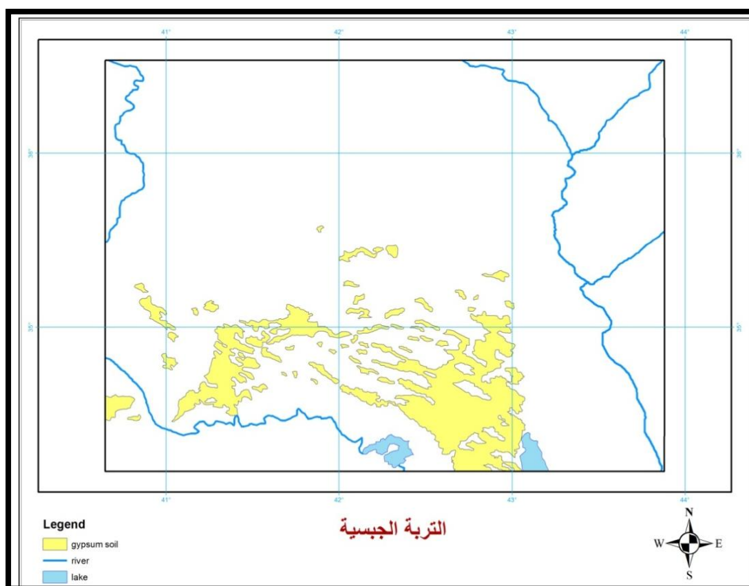
Fig. 5. Map for gypsiferous soil in north-west of Iraq
