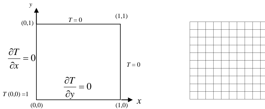
Fig. 2. Heat conduction problem: (a) boundary conditions, (b) FE grid
