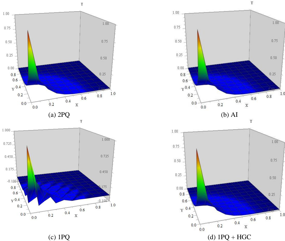
Fig. 3. Heat-conduction problem with the boundary condition T = 1.0 at (0,0) : solutions with (a) 2PQ, (b) AI, (c) 1PQ without HGC and (d) 1PQ with HGC.
