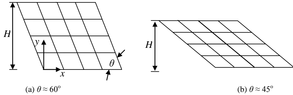
Fig. 5. Heat conduction problem in a skewed domain
