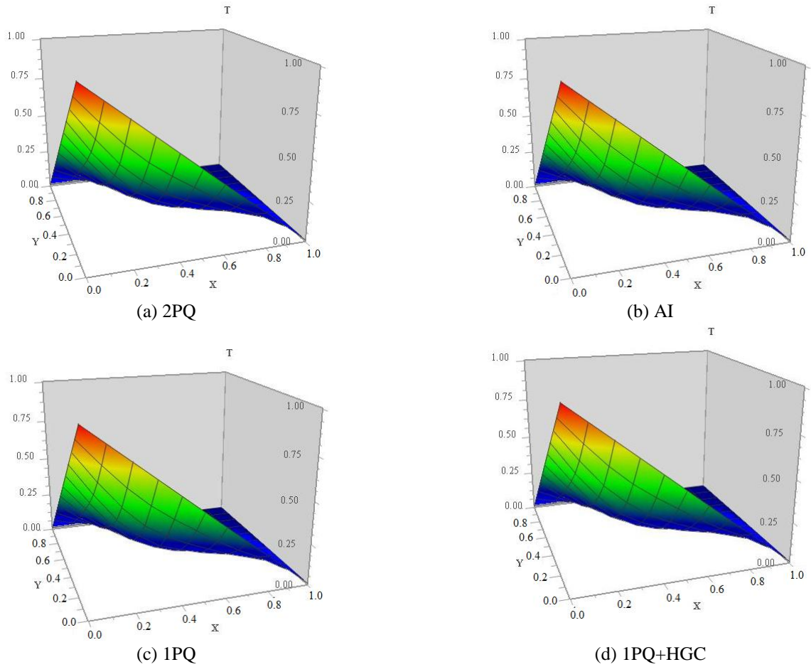
Fig. 4. Heat-conduction problem with boundary condition ( T = 1-x ) at y=0 and ( T = 1-y ) at x=0 : solutions with (a) 2PQ, (b) AI, (c) 1PQ without HGC and (d) 1PQ with HGC.
