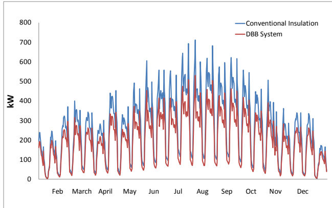
Fig (6). Chiller Power Consumption Comparison
