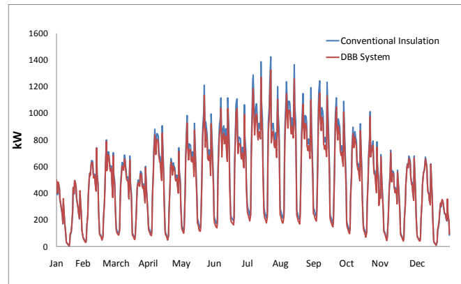
Fig (5). Cooling Load Demand Comparison
