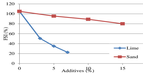
Fig. 2. Additives contents on soil versus free swell index.
