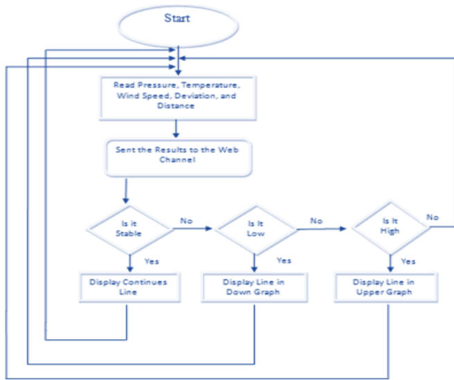
Figure.4: Algorithm
