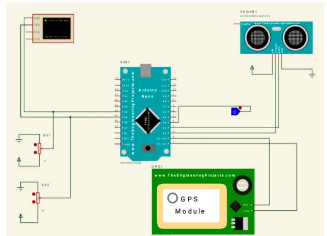
Figure.2: Circuit schematic
