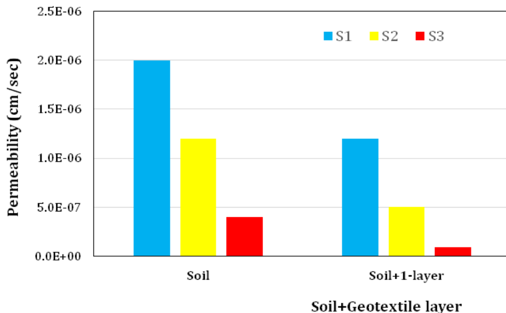
Fig.5. Permeability of natural and reinforced soils with geotextile
