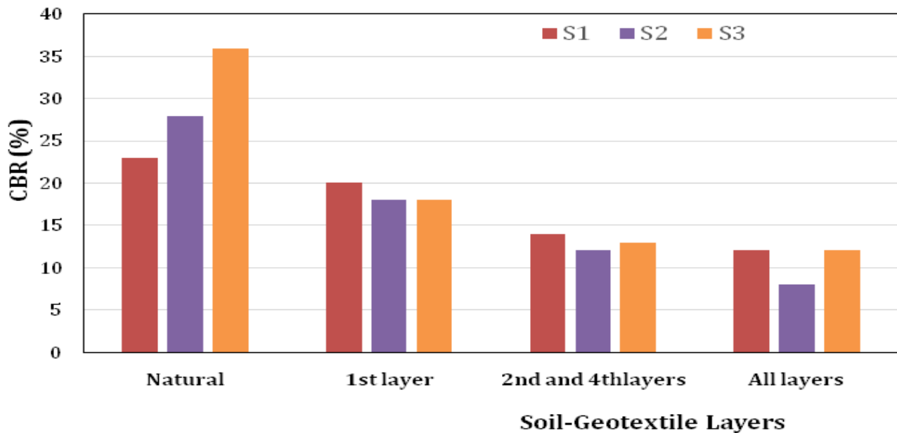
Fig.4. CBR values for natural and reinforced soils with geotextile layers
