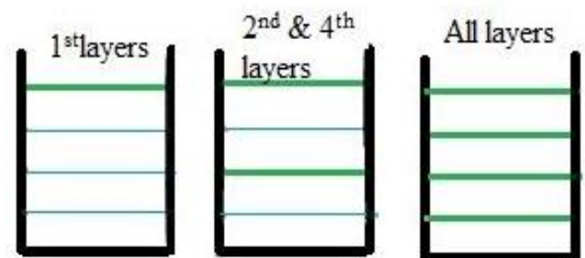
Fig.3. Simple sketches of specimens with geotextile sheets placed between soil layers
