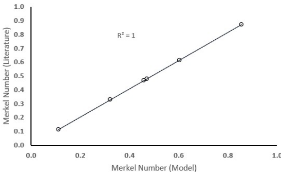
Figure 3: Merkel Number [18]
